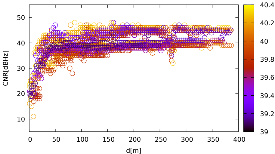
CNR vs distance (UbloxF9R for C13 at L1)
