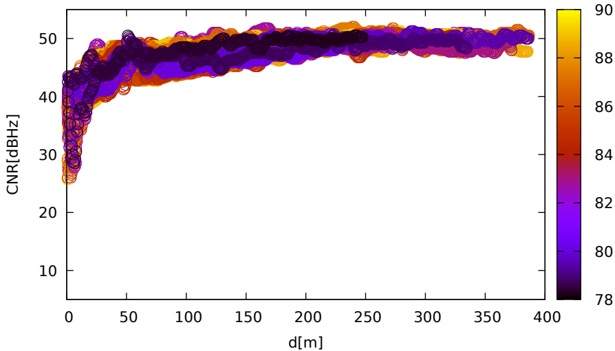
CNR vs distance (LeicaGS18 for R21 at L1)
