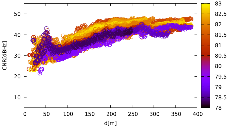
CNR vs distance (Javad for G29 at L1)
