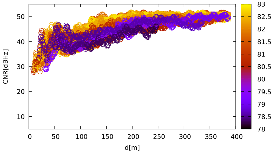
CNR vs distance (LeicaGS15 for G29 at L1)
