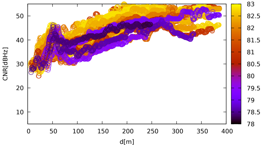
CNR vs distance (LeicaGS18 for G29 at L1)
