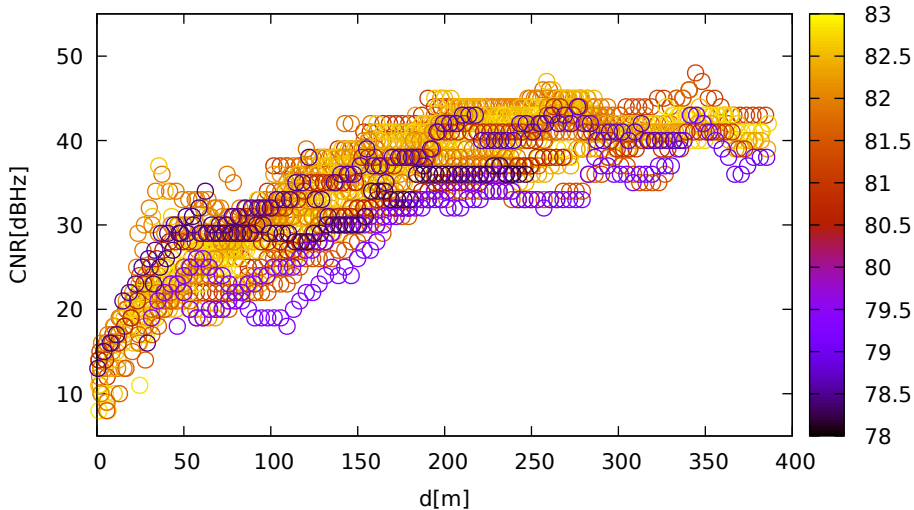
CNR vs distance (UbloxF9R for G29 at L1)
