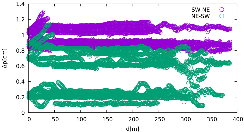
Position displacement vs. jammer distance (Javad on GLONASS)
