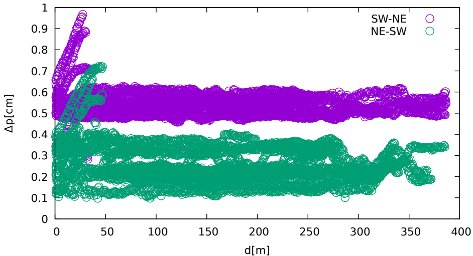
Position displacement vs. jammer distance (Javad on GPS/GLONASS)
