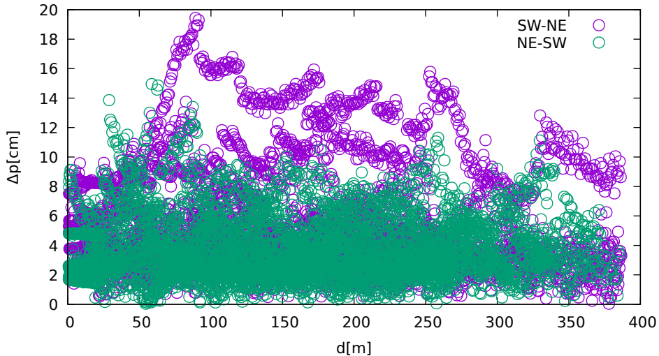
Position displacement vs. jammer distance (Javad on GPS/GLONASS/Galileo/BeiDou)
