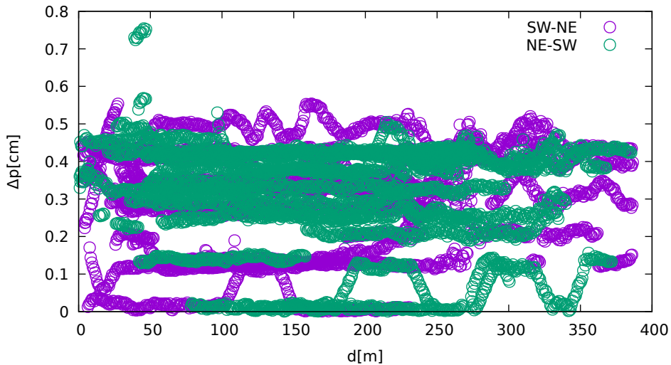
Position displacement vs. jammer distance (LeicaGS18 on BeiDou)
