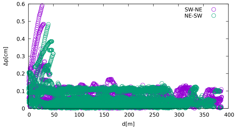
Position displacement vs. jammer distance (LeicaGS18 on GPS/GLONASS/Galileo/BeiD)
