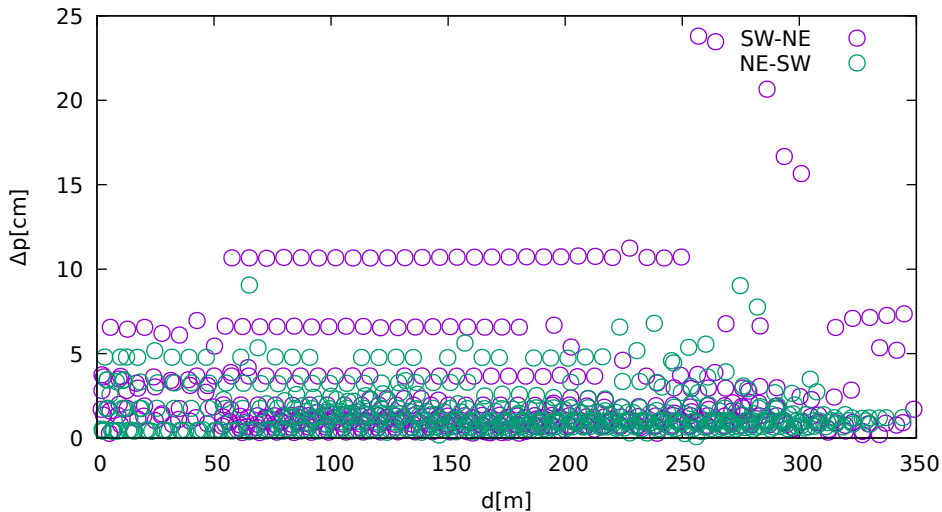
Position displacement vs. jammer distance (Ublox8T on GLONASS)
