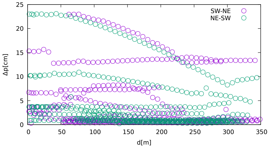
Position displacement vs. jammer distance (Ublox8T on GPS/GLONASS/Galileo/BeiDou)
