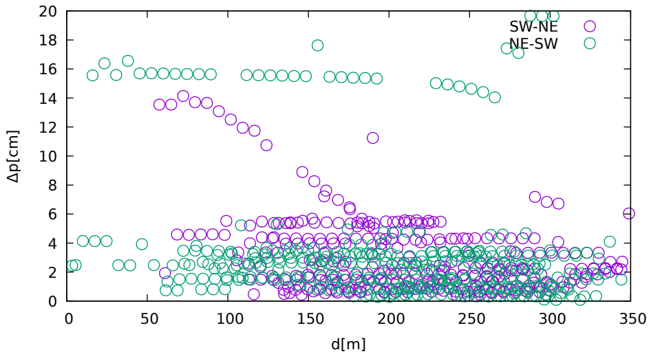
Position displacement vs. jammer distance (Ublox8T on Galileo)
