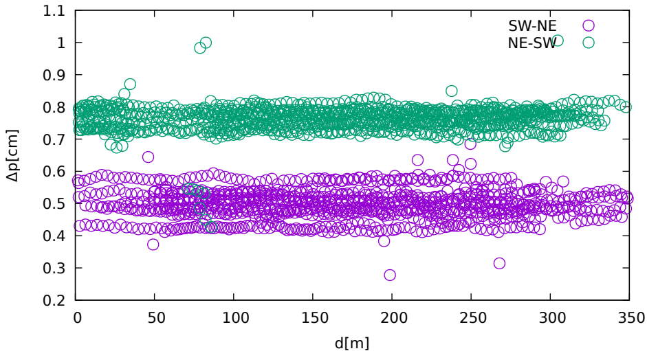
Position displacement vs. jammer distance (UbloxF9P on GPS/GLONASS)
