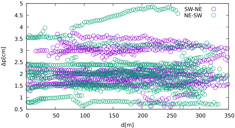
Position displacement vs. jammer distance (UbloxF9P on GPS/GLONASS/Galileo)
