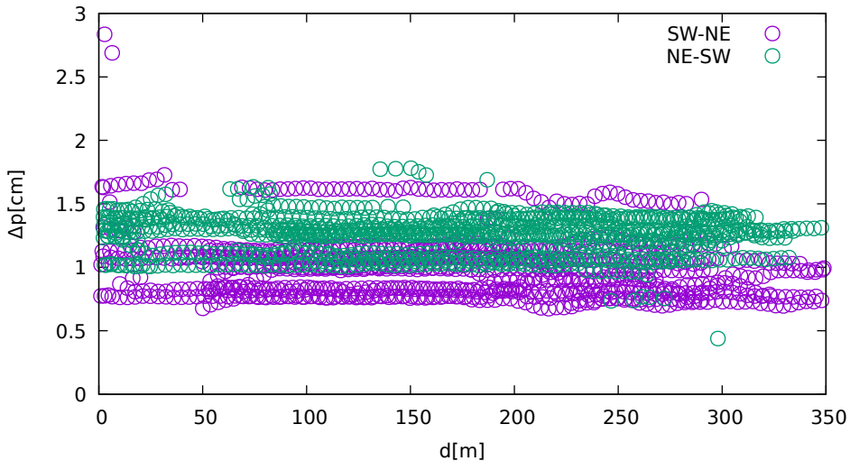
Position displacement vs. jammer distance (UbloxF9R on GPS/GLONASS)
