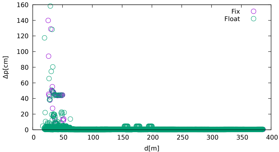
Position displacement vs. jammer distance (Javad on GPS/Galileo)
