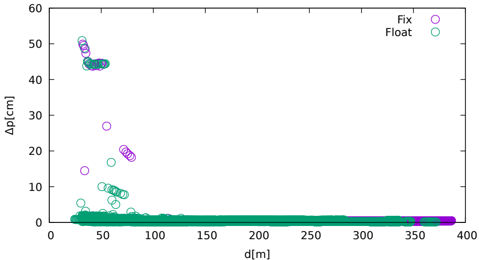
Position displacement vs. jammer distance (Javad on Galileo)
