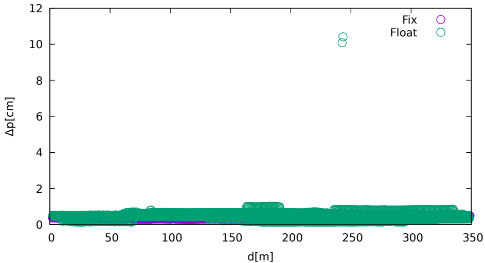
Position displacement vs. jammer distance (LeicaGS15 on GLONASS)
