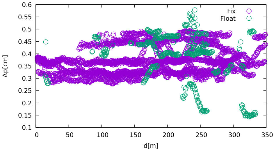
Position displacement vs. jammer distance (LeicaGS15 on Galileo)
