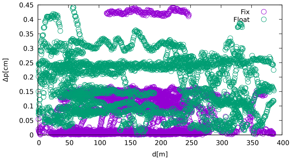
Position displacement vs. jammer distance (LeicaGS18 on GLONASS)
