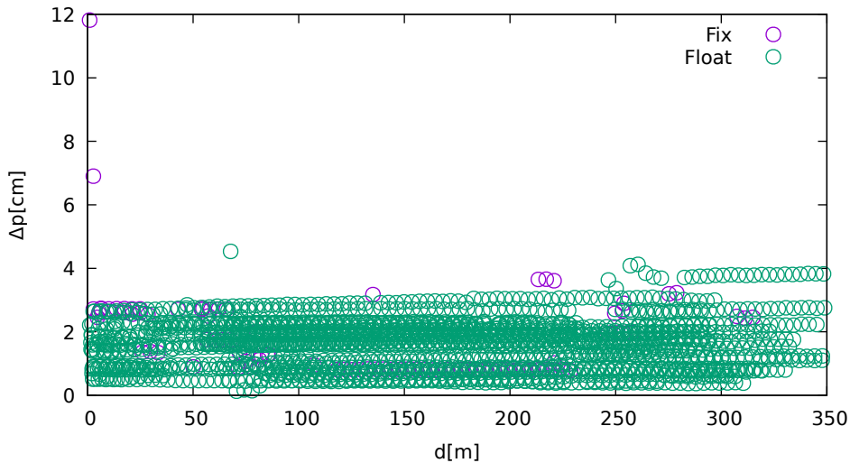
Position displacement vs. jammer distance (UbloxF9P on BeiDou)
