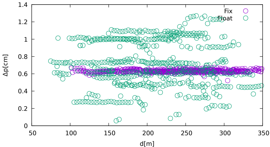
Position displacement vs. jammer distance (UbloxF9P on GPS)
