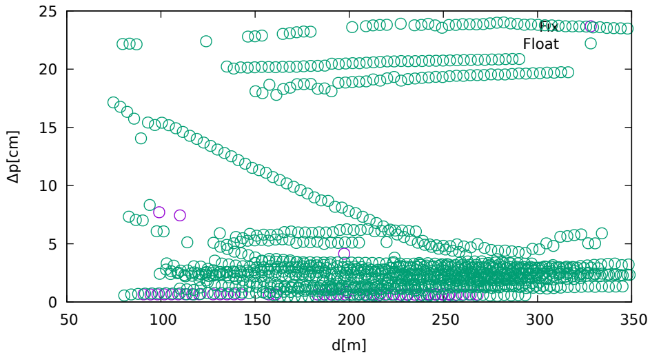
Position displacement vs. jammer distance (UbloxF9P on GPS/Galileo)
