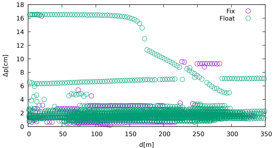
Position displacement vs. jammer distance (UbloxF9R on BeiDou)
