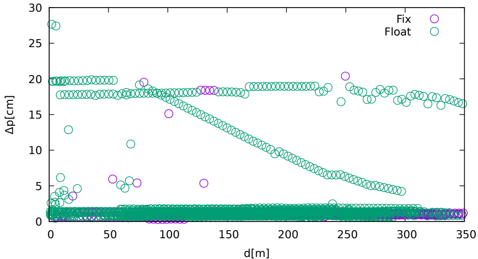
Position displacement vs. jammer distance (UbloxF9R on GPS)
