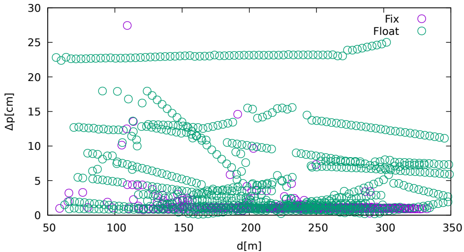
Position displacement vs. jammer distance (UbloxF9R on GPS/Galileo)
