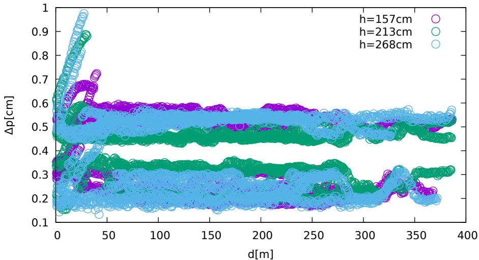
Position displacement vs. jammer distance (Javad on GPS/GLONASS/Galileo)
