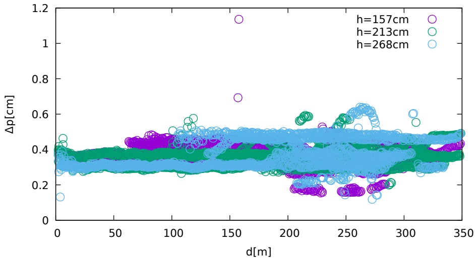
Position displacement vs. jammer distance (LeicaGS15 on GPS)
