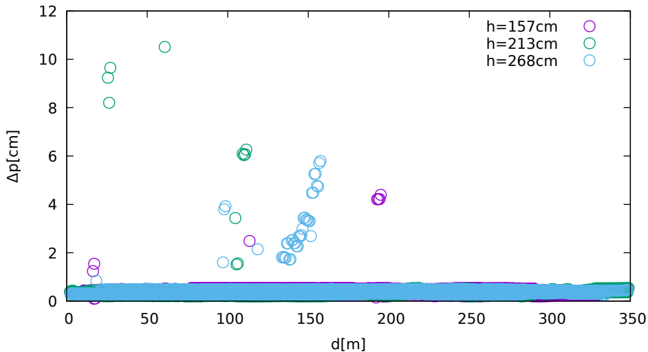
Position displacement vs. jammer distance (LeicaGS15 on GPS/GLONASS/Galileo)
