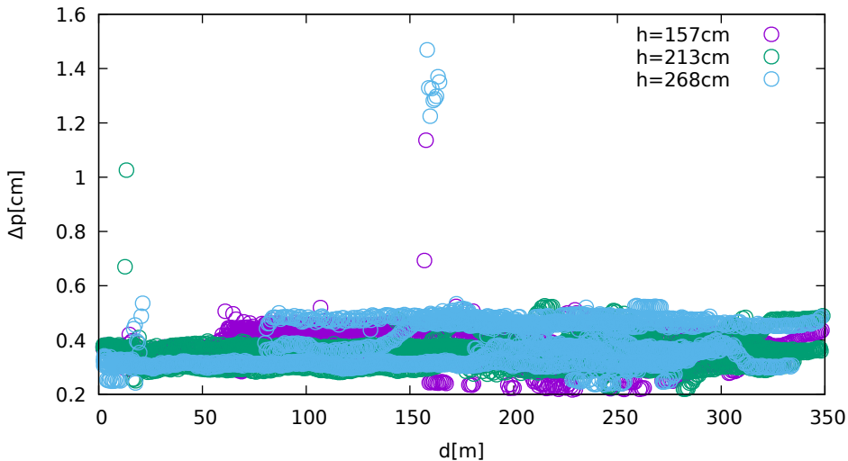
Position displacement vs. jammer distance (LeicaGS15 on GPS/Galileo)
