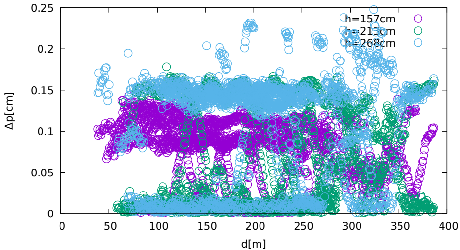
Position displacement vs. jammer distance (LeicaGS18 on GPS)
