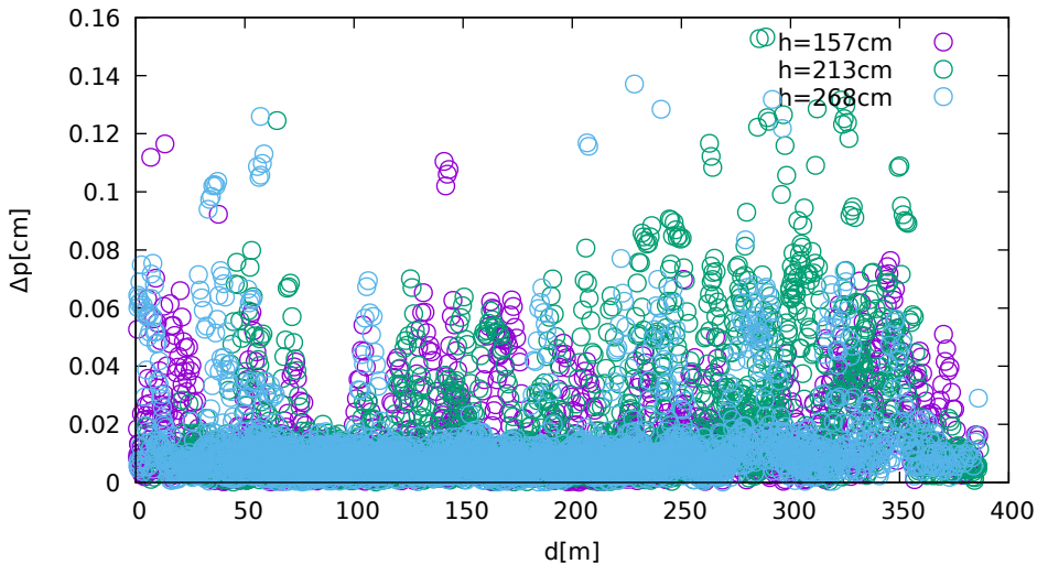
Position displacement vs. jammer distance (LeicaGS18 on GPS/GLONASS)
