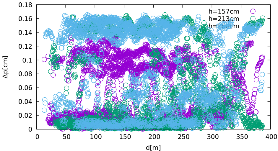
Position displacement vs. jammer distance (LeicaGS18 on GPS/Galileo)
