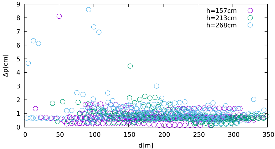
Position displacement vs. jammer distance (Ublox8T on GPS)
