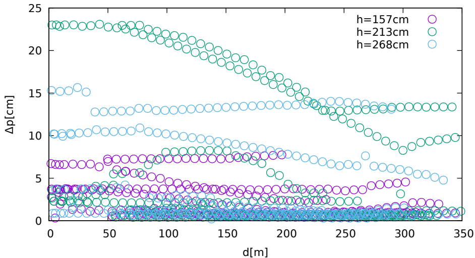
Position displacement vs. jammer distance (Ublox8T on GPS/GLONASS/Galileo)
