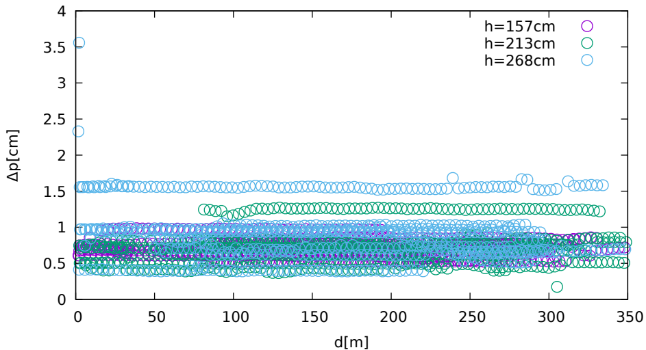
Position displacement vs. jammer distance (UbloxF9P on GLONASS)
