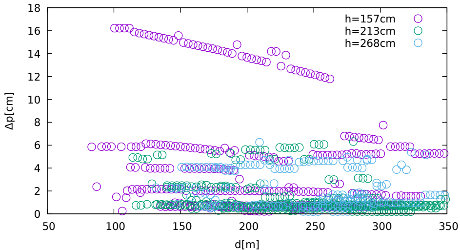
Position displacement vs. jammer distance (UbloxF9P on Galileo)
