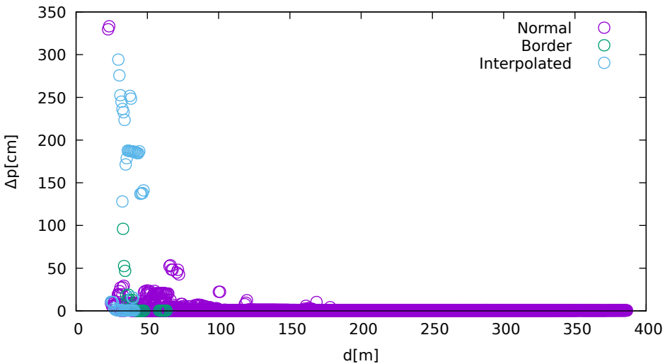
Position displacement vs. jammer distance (Javad on GPS)
