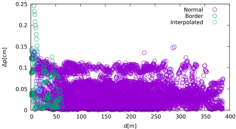
Position displacement vs. jammer distance (LeicaGS18 on GPS/GLONASS/Galileo)
