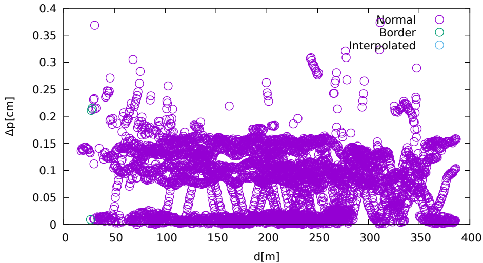
Position displacement vs. jammer distance (LeicaGS18 on Galileo)
