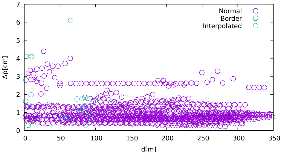
Position displacement vs. jammer distance (Ublox8T on GPS/GLONASS)
