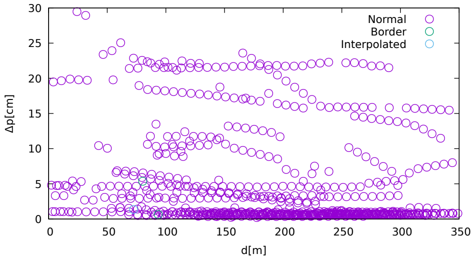
Position displacement vs. jammer distance (Ublox8T on GPS/Galileo)
