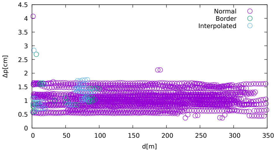
Position displacement vs. jammer distance (UbloxF9R on GLONASS)
