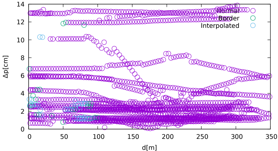
Position displacement vs. jammer distance (UbloxF9R on GPS/GLONASS/Galileo)
