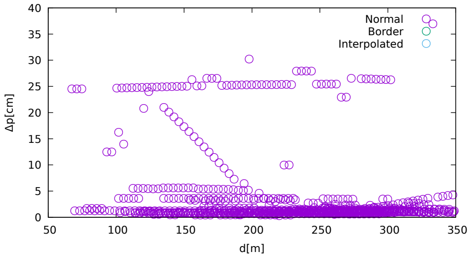
Position displacement vs. jammer distance (UbloxF9R on Galileo)
