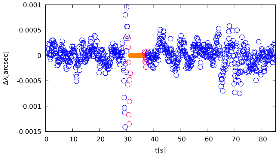
Position difference (N direction)
