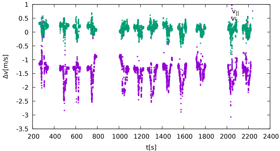
Difference between Doppler and interpolated speed (Javad)
