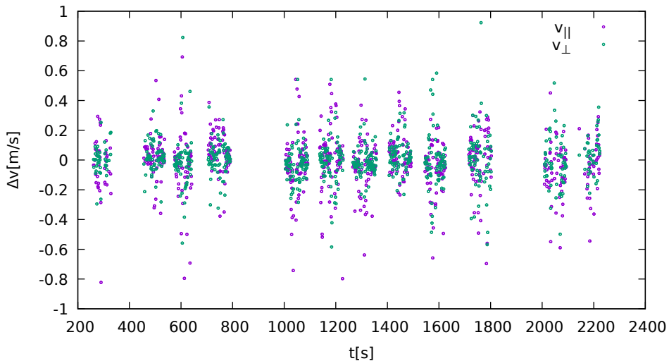
Difference between Doppler and interpolated speed (Ublox8T)
